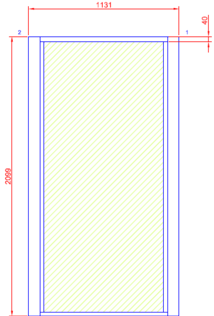
Front and back sides dimensions
